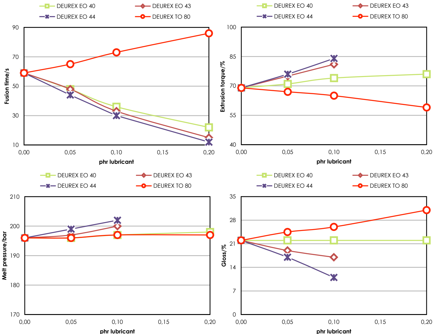
Fig. 1 to Fig. 4 Influence of the dosage of DEUREX® EO 43 in comparison to EO 40, EO 44 and TO 80 on fusion time (Fig. 1), extrusion torque (Fig. 2), melt pressure (Fig. 3) and gloss (Fig. 4)
